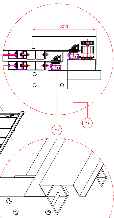
DETAIL :A
