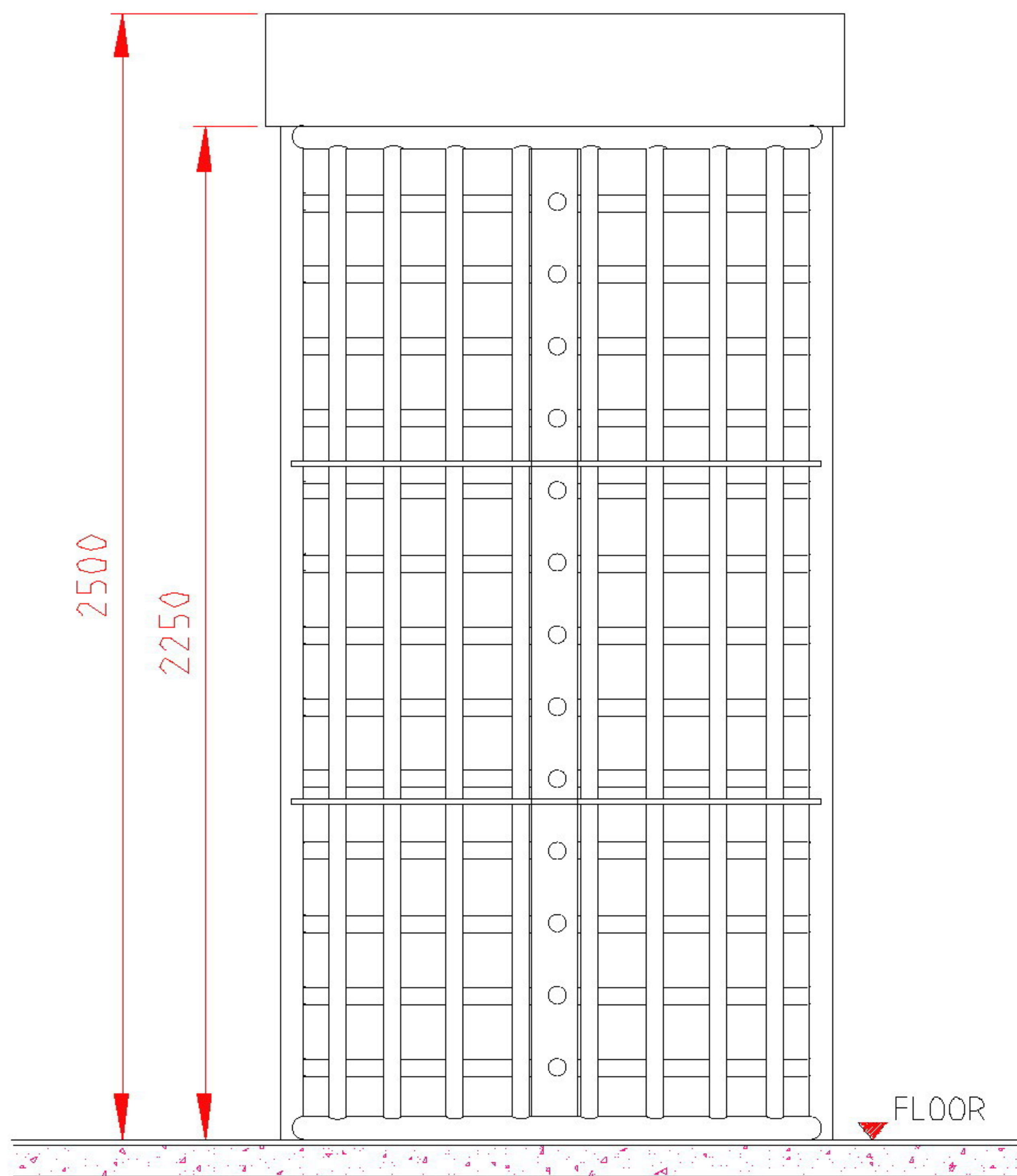
FRONT VIEW
