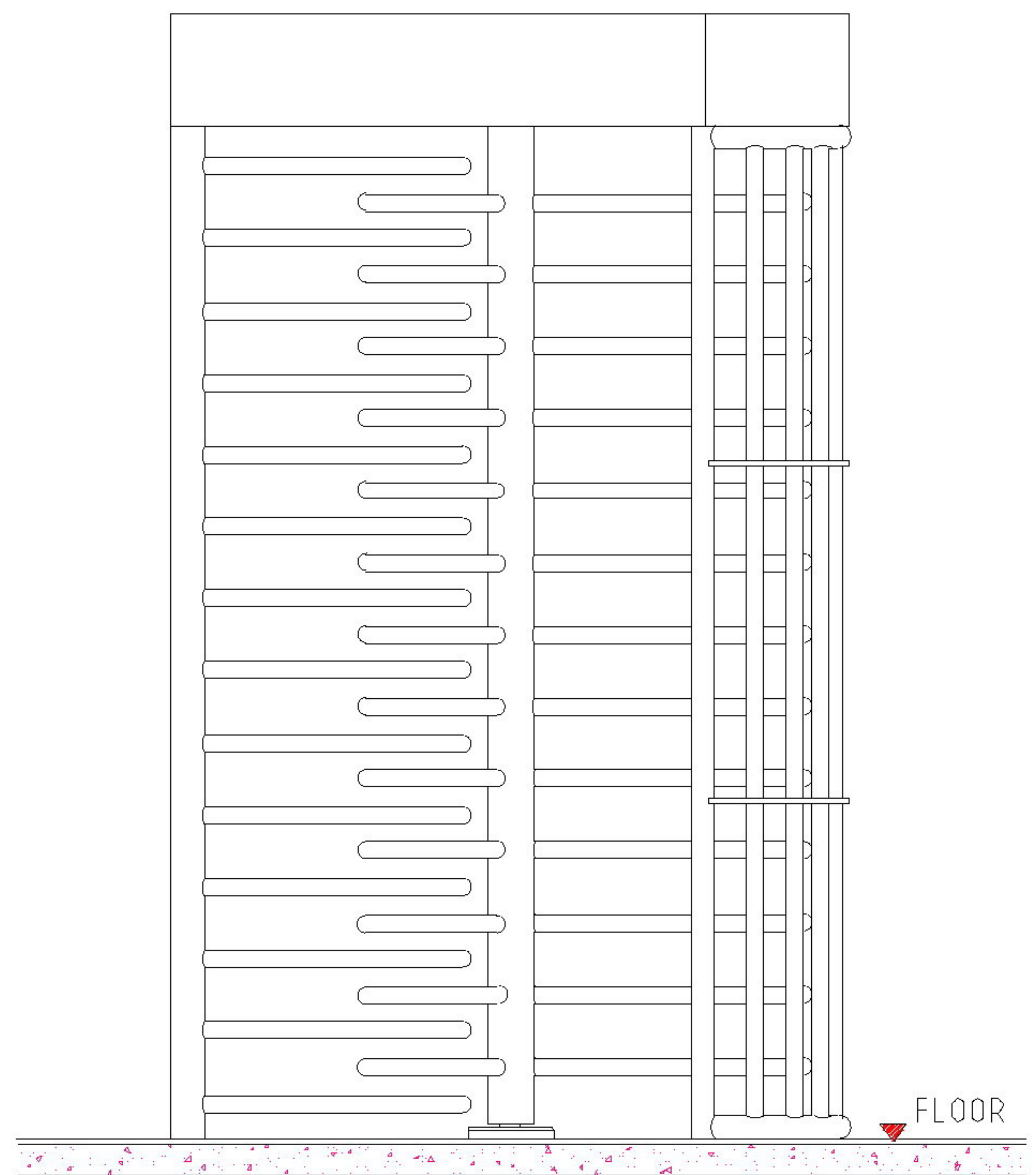
SIDE VIEW
